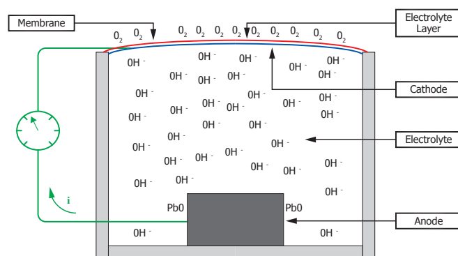
Sensor Construction
